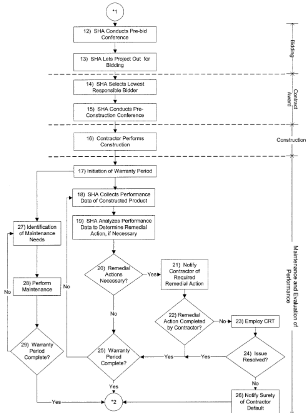
Figure CA-8.1 (continued): Flowchart process model for warranty contracting (from Anderson and Russell 2001).
