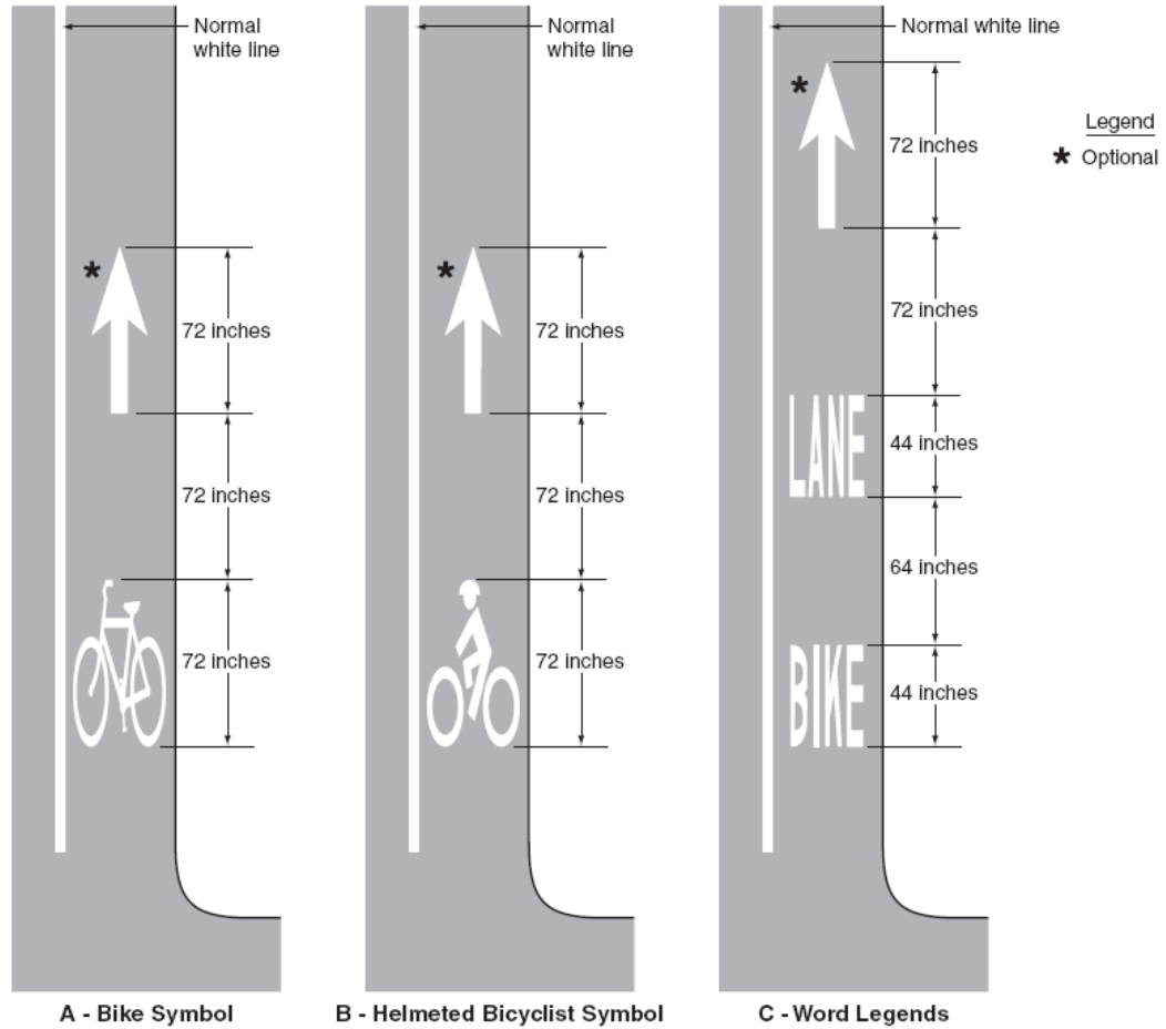
Figure AE-6.2: Examples of dedicated lanes for bicycle access. 2 points if new or improved to meet or exceed these minimum dimensions. (FHWA, 2009)
