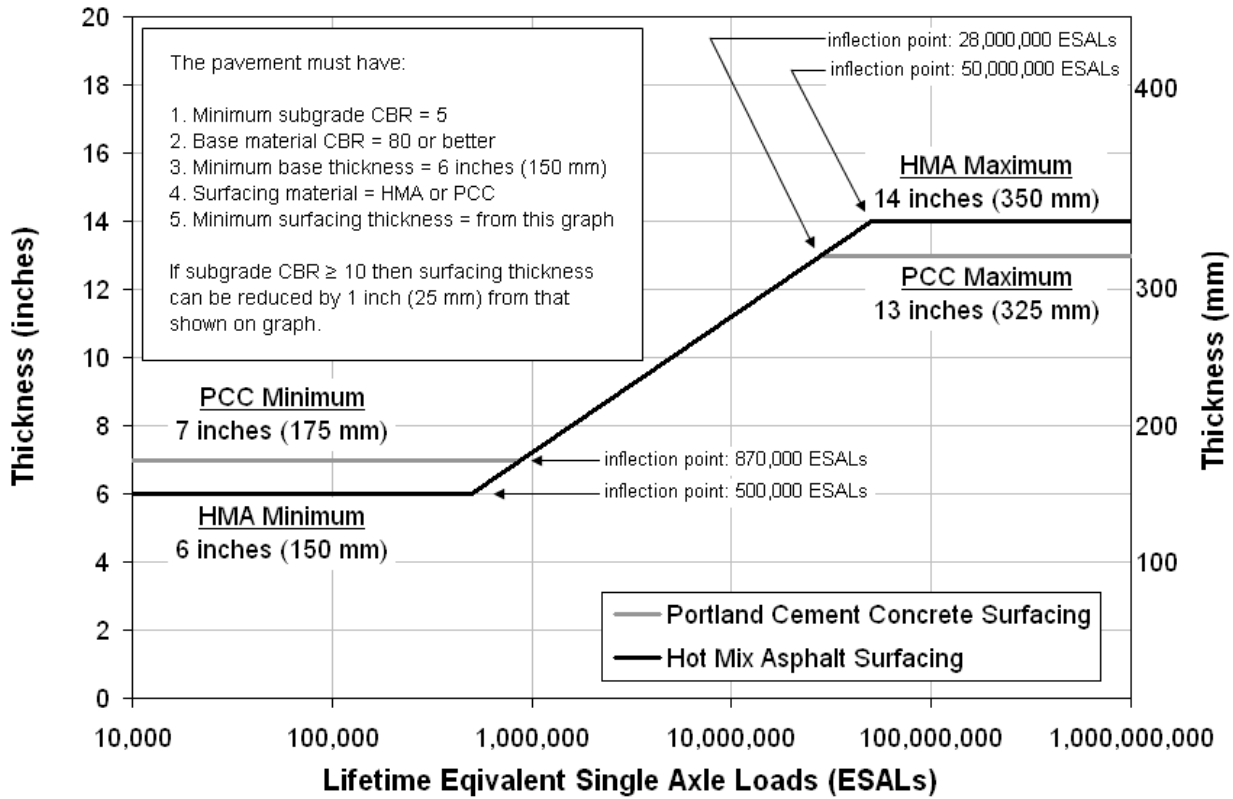
Figure PT-1.1: Long-life pavement design graph.
