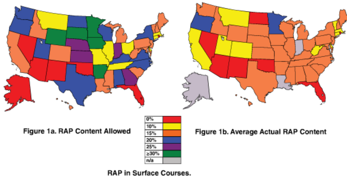
Figure MR-4.10: RAP use in HMA surface courses (from Newcomb and Jones, 2008).
