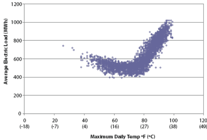
Figure PT-4.2: Increasing electrical loads with increasing temperatures. This is an example of New Orleans from Sailor (2002).
