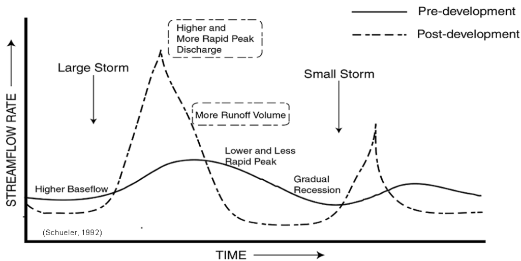
Figure 1.1 – Changes in Hydrology After Development
