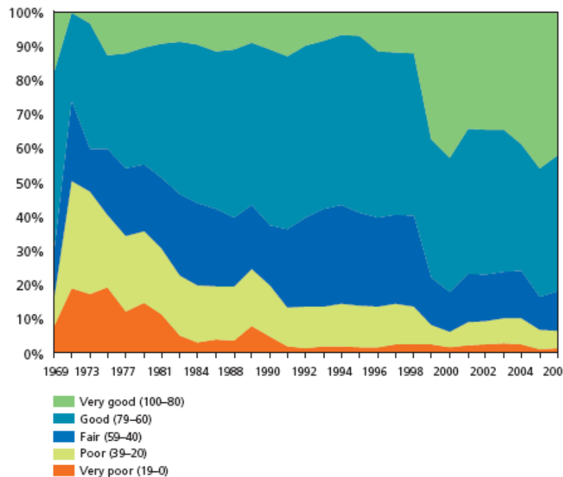
Figure PR-10.2: Trends in Washington State pavement structural condition, 1969–2006 from FHWA (2008). Data source: Washington State Department of Transportation Materials Laboratory.
