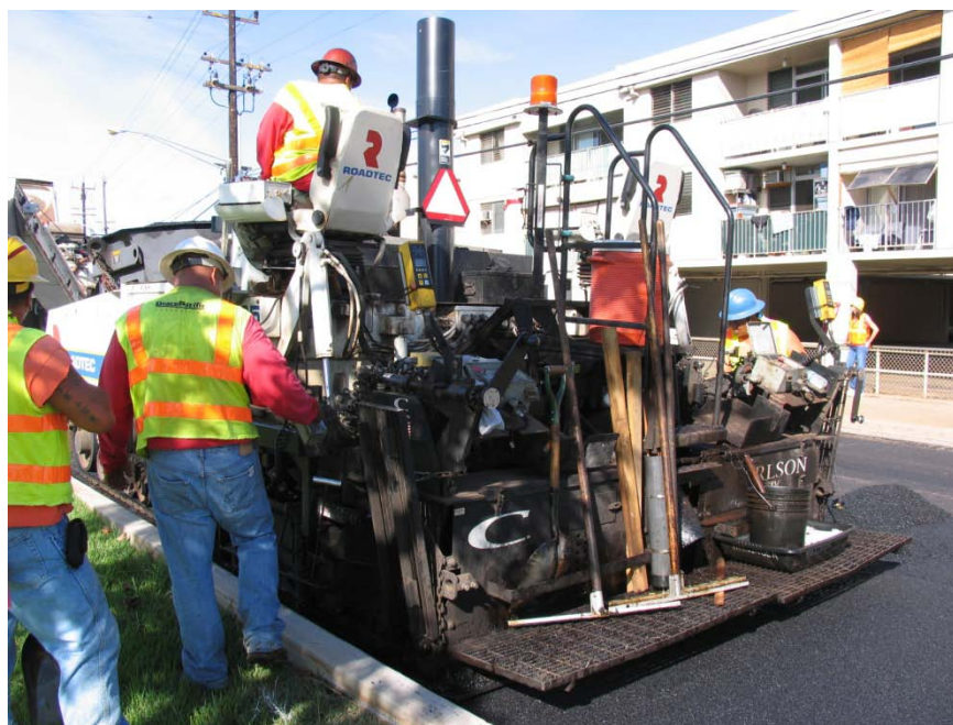
Figure CA-6.2: The large black exhaust stack to the right of the operator is part of a NIOSH compliant exhaust ventilation system.
