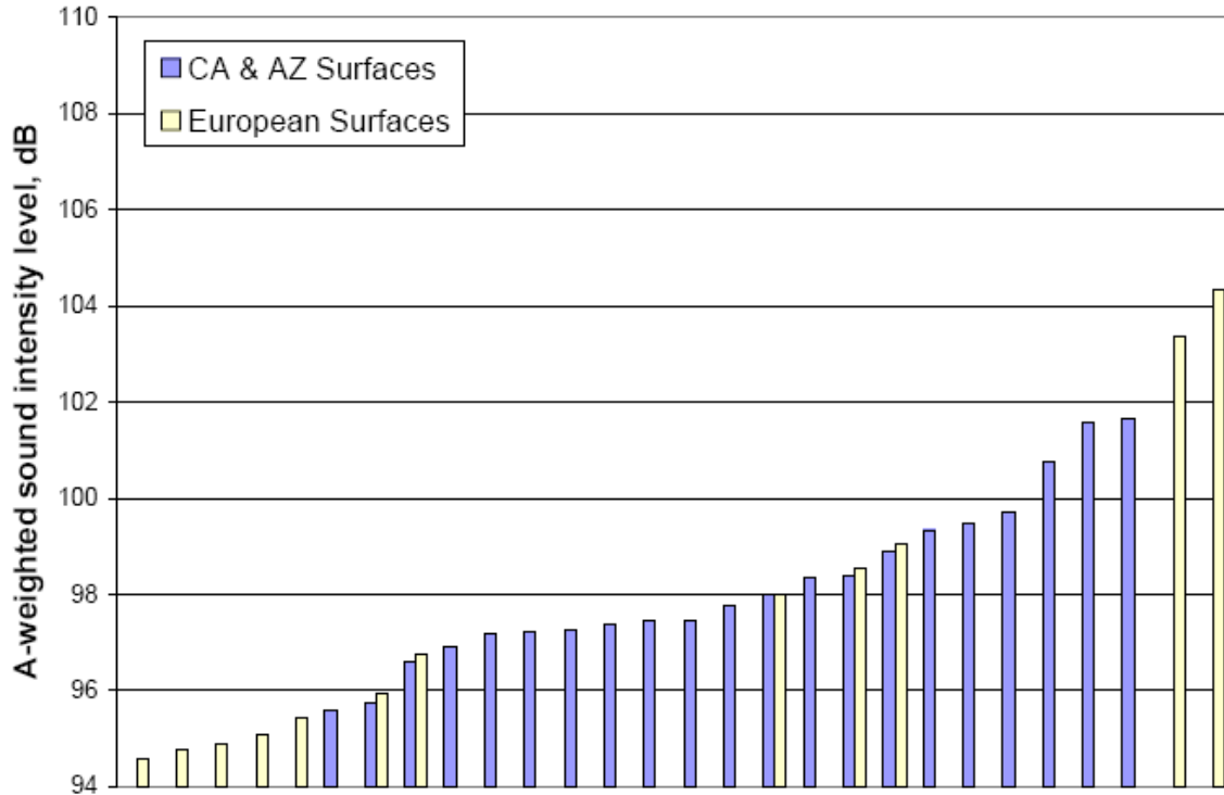
Figure PT-5.4: Comparison of sound intensity levels for various types of HMA open-graded surface courses in California, Arizona and Europe at 97 km/hr (60 mph). From Donovan, no date given.
