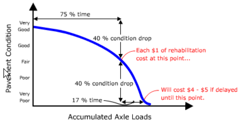
Figure PR-10.4: Rehabilitation time vs. cost (based on an illustration in Stevens, 1985).
