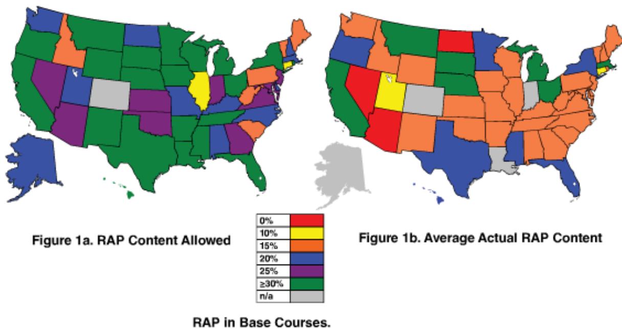
Figure MR-4.9: RAP use in HMA base courses (from Newcomb and Jones, 2008).
