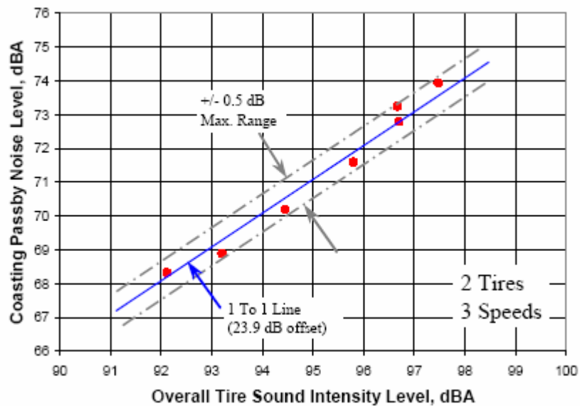
Figure PT-5.3: Relationship between pass-by (roadside) measurements and OBSI measurements for one particular study (graph from Donovan and Rymer, 2003).
